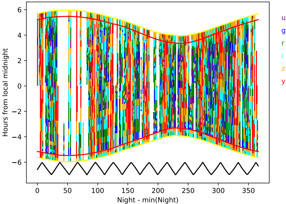
too_elab_r8_d2_griz_v3.4_10yrs year 3-4: Hourglass
