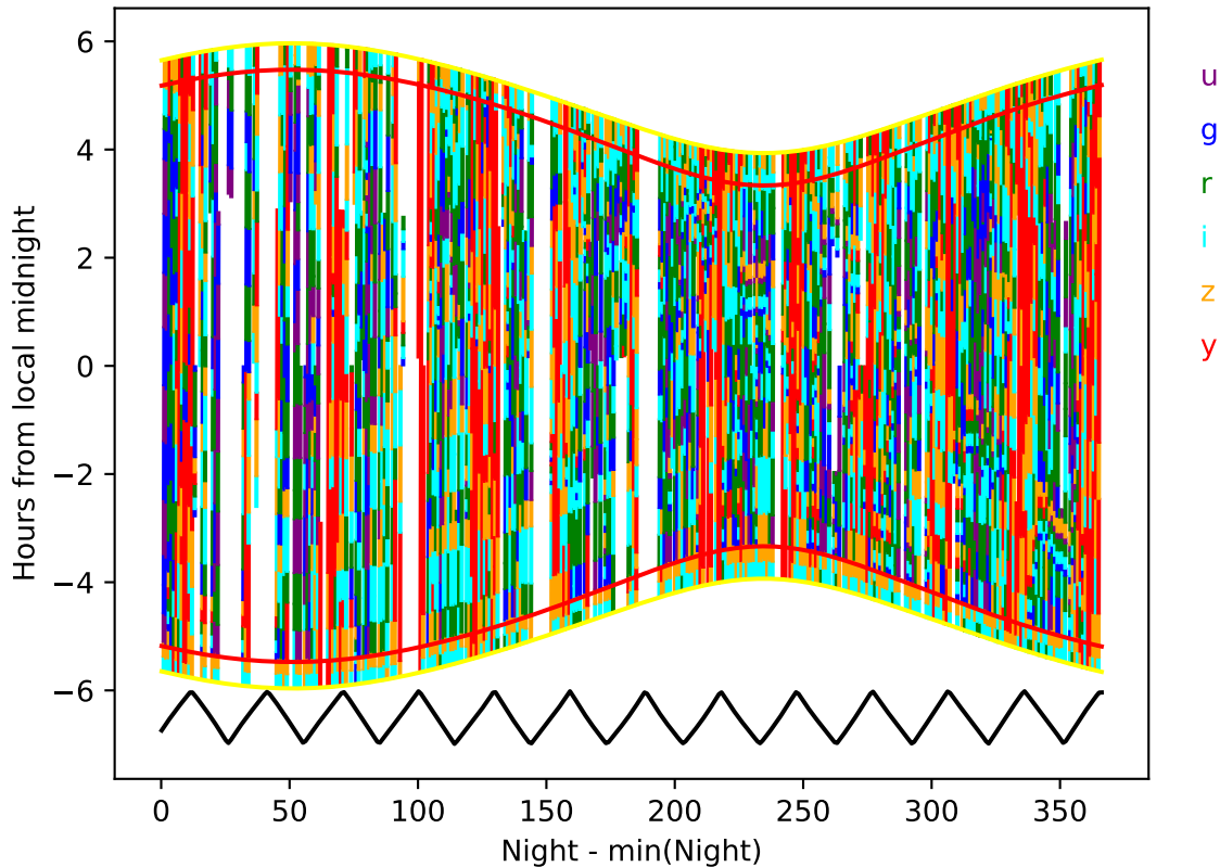
too_elab_r8_d2_griz_v3.4_10yrs year 0-1: Hourglass
