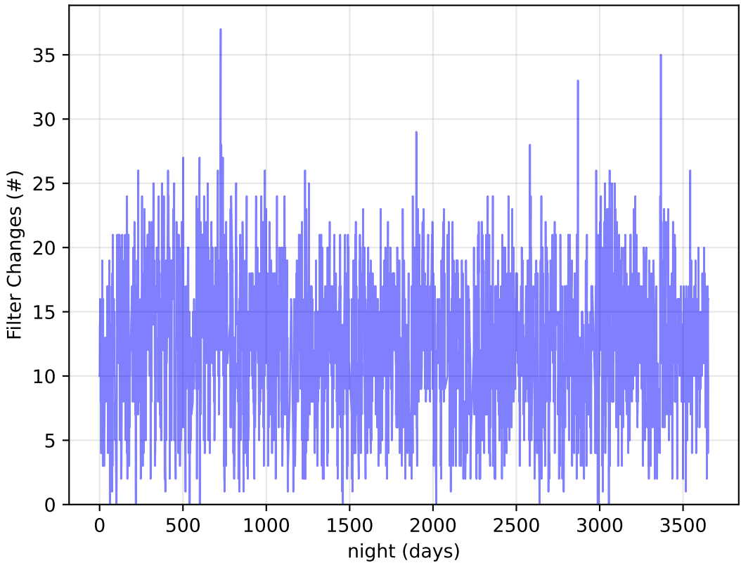
too_elab_r8_d2_griz_v3.4_10yrs : Filter Changes
