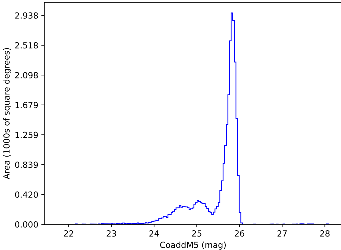
too_elab_r8_d2_griz_v3.4_10yrs z: CoaddM5
