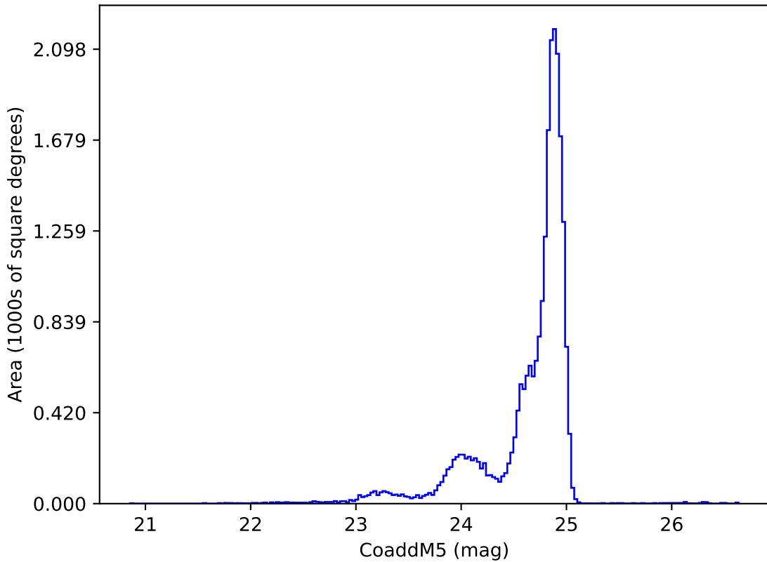
too_elab_r8_d2_griz_v3.4_10yrs y: CoaddM5
