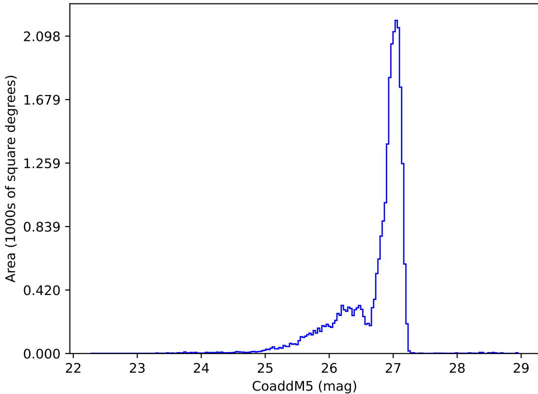
too_elab_r8_d2_griz_v3.4_10yrs r: CoaddM5
