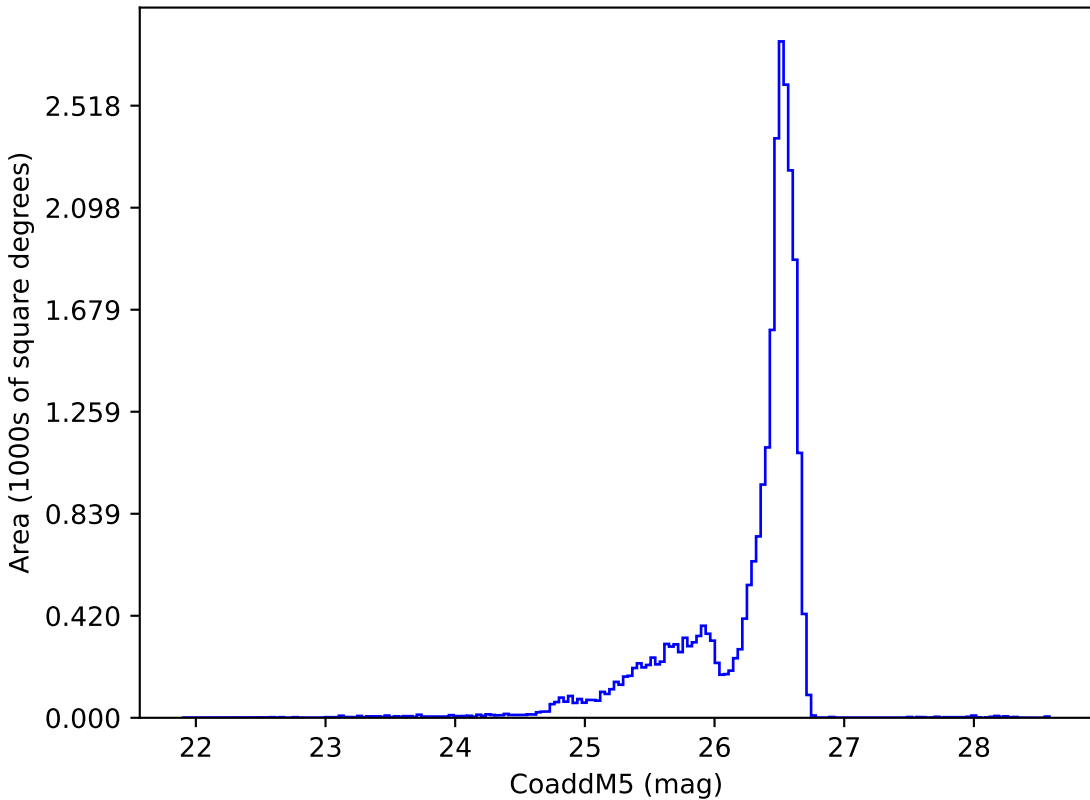
too_elab_r8_d2_griz_v3.4_10yrs i: CoaddM5
