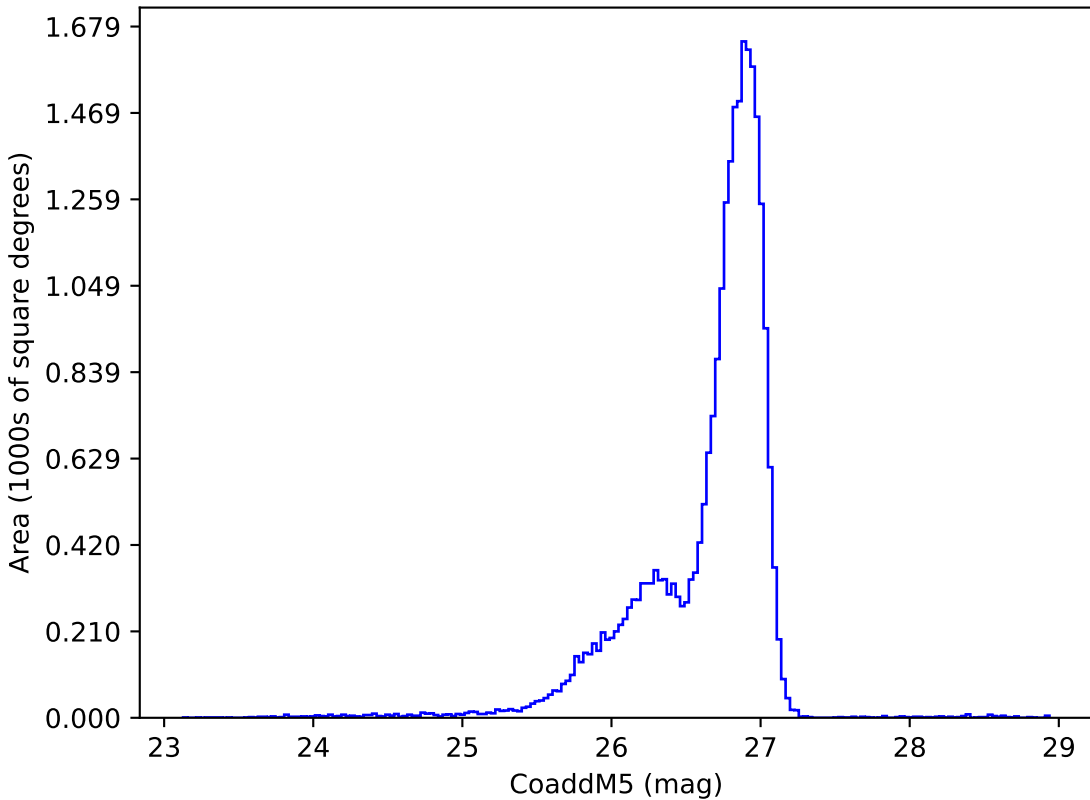
too_elab_r8_d2_griz_v3.4_10yrs g: CoaddM5
