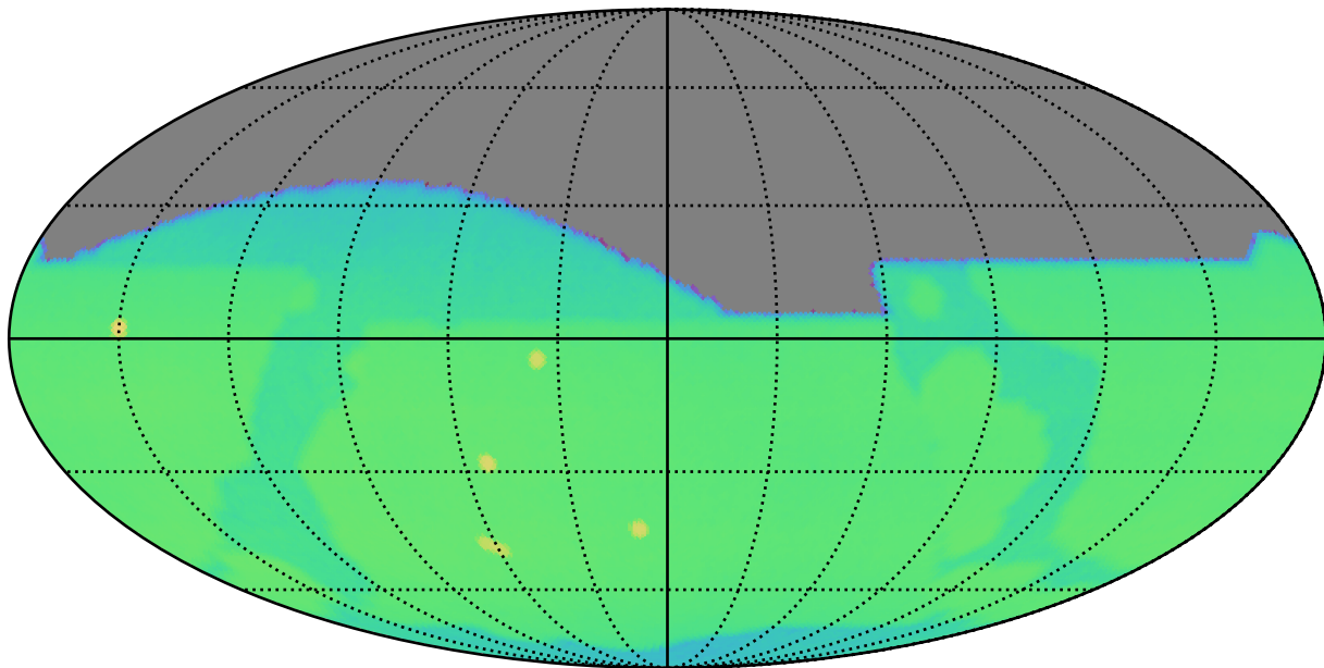
too_elab_r8_d2_griz_v3.4_10yrs : CoaddM5
