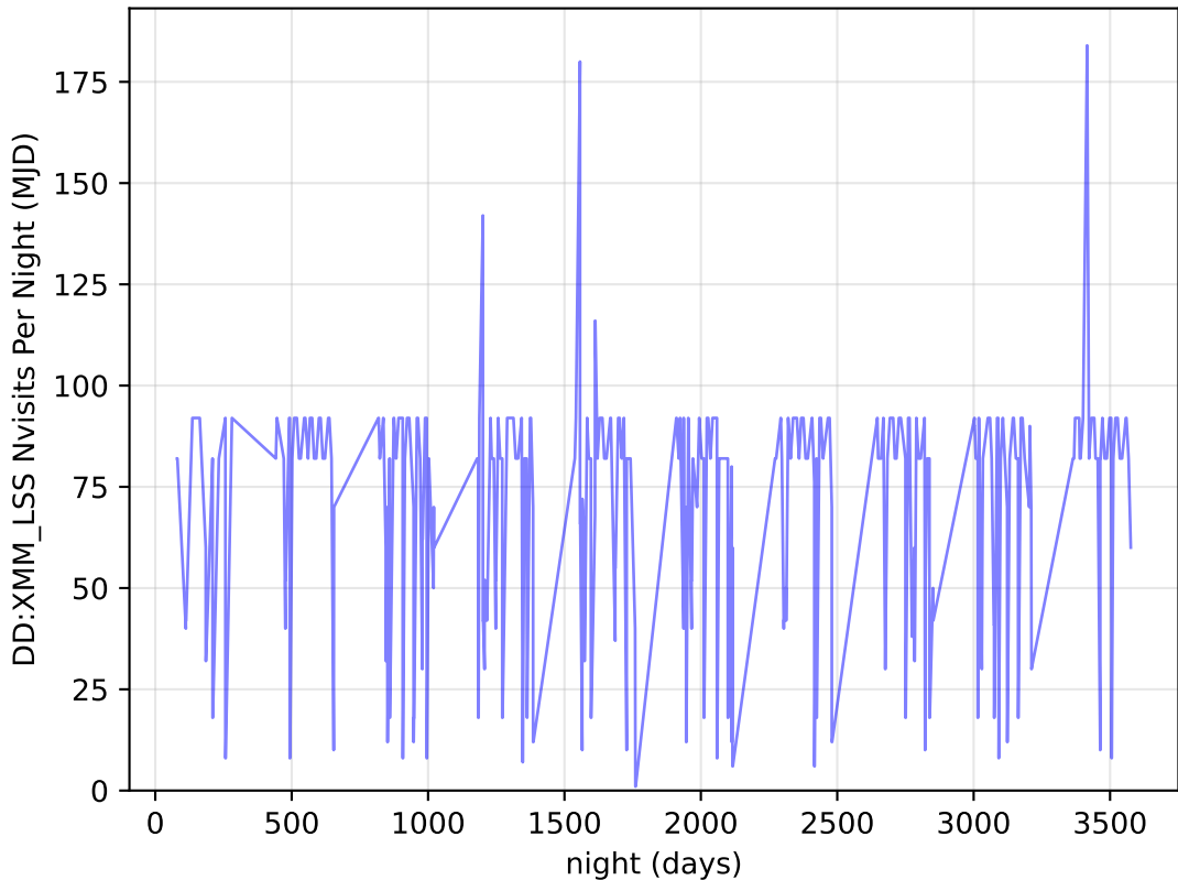
too_elab_r8_d2_griz_v3.4_10yrs all bands: DD:XMM_LSS Nvisits Per Night
