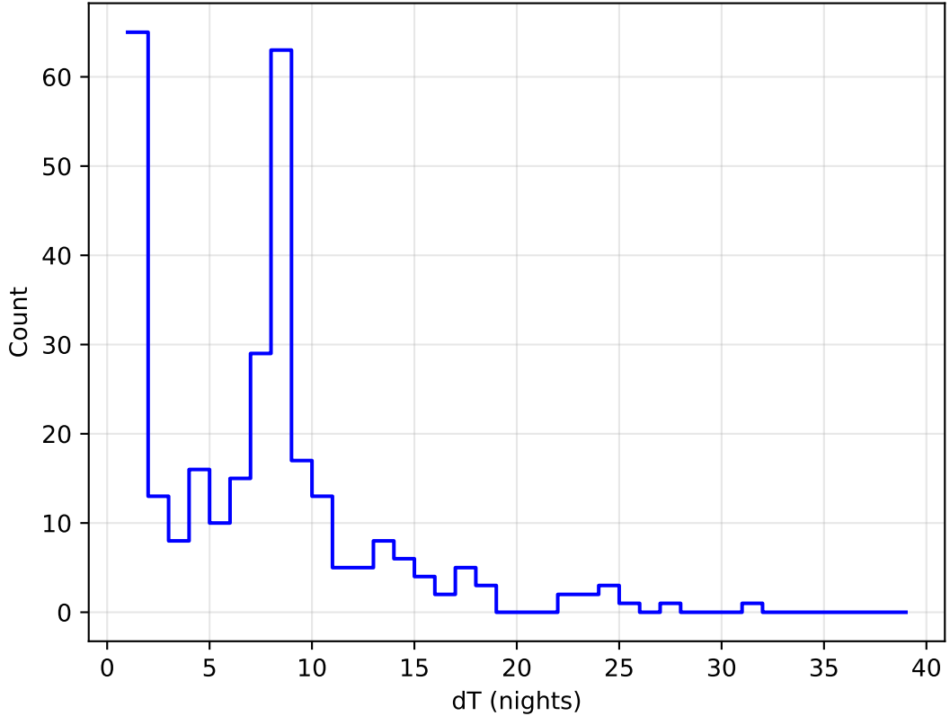
too_elab_r8_d2_griz_v3.4_10yrs all bands: DD:XMM_LSS Delta Nights Histogram
