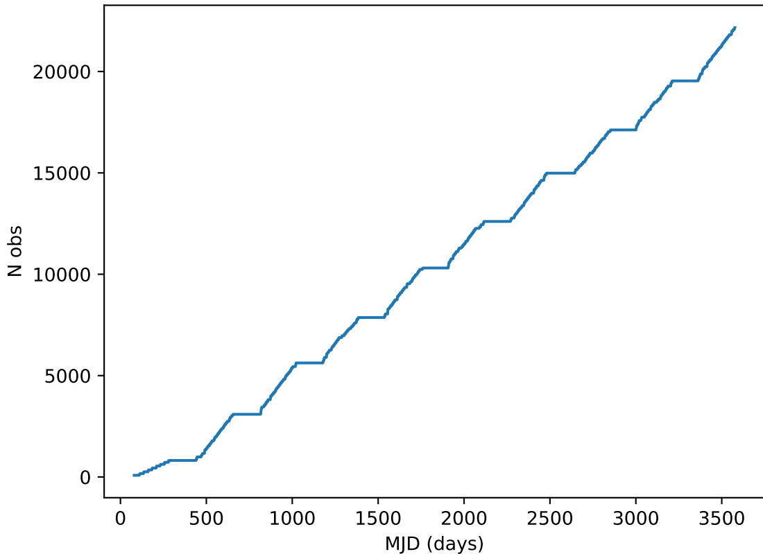
too_elab_r8_d2_griz_v3.4_10yrs all bands: DD:XMM_LSS Cumulative NVisits
