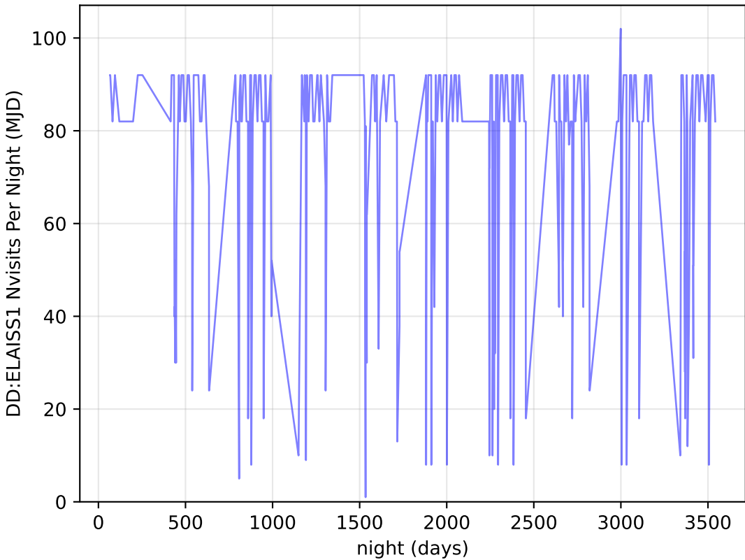
too_elab_r8_d2_griz_v3.4_10yrs all bands: DD:ELAISS1 Nvisits Per Night
