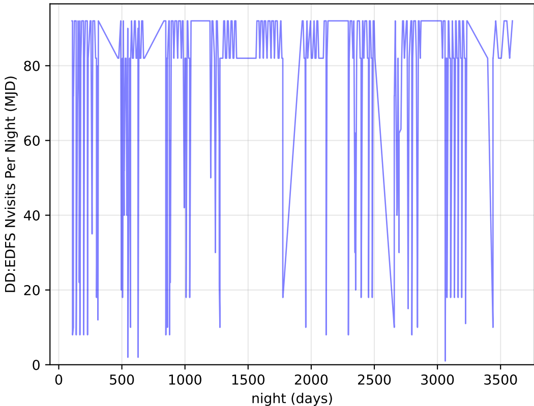
too_elab_r8_d2_griz_v3.4_10yrs all bands: DD:EDFS Nvisits Per Night
