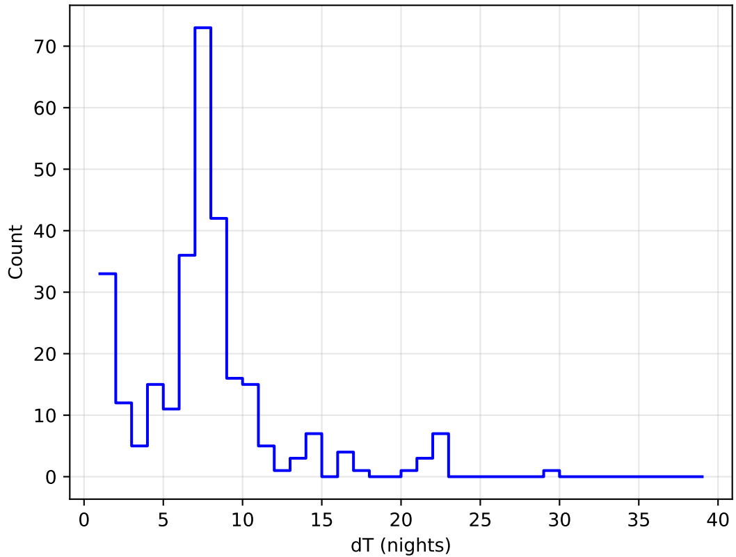
too_elab_r8_d2_griz_v3.4_10yrs all bands: DD:EDFS Delta Nights Histogram
