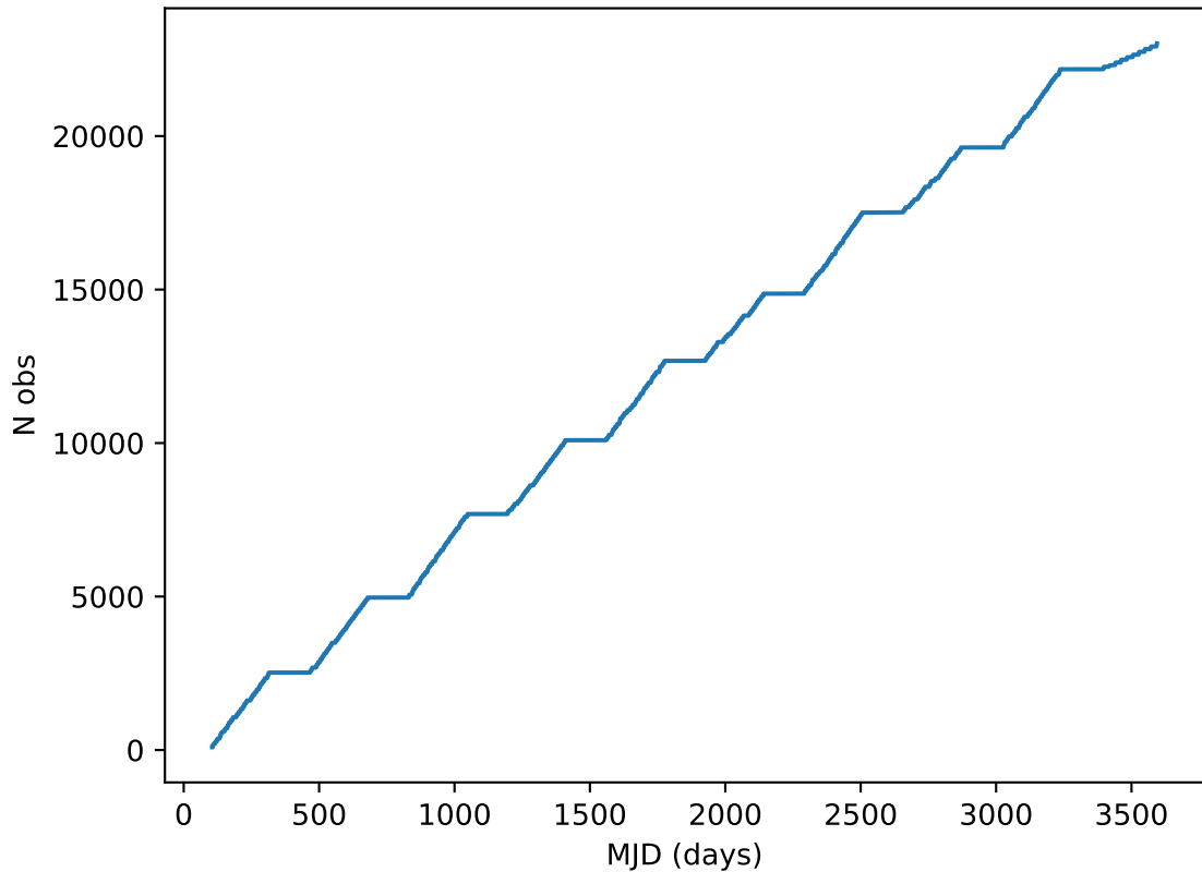
too_elab_r8_d2_griz_v3.4_10yrs all bands: DD:EDFS Cumulative NVisits
