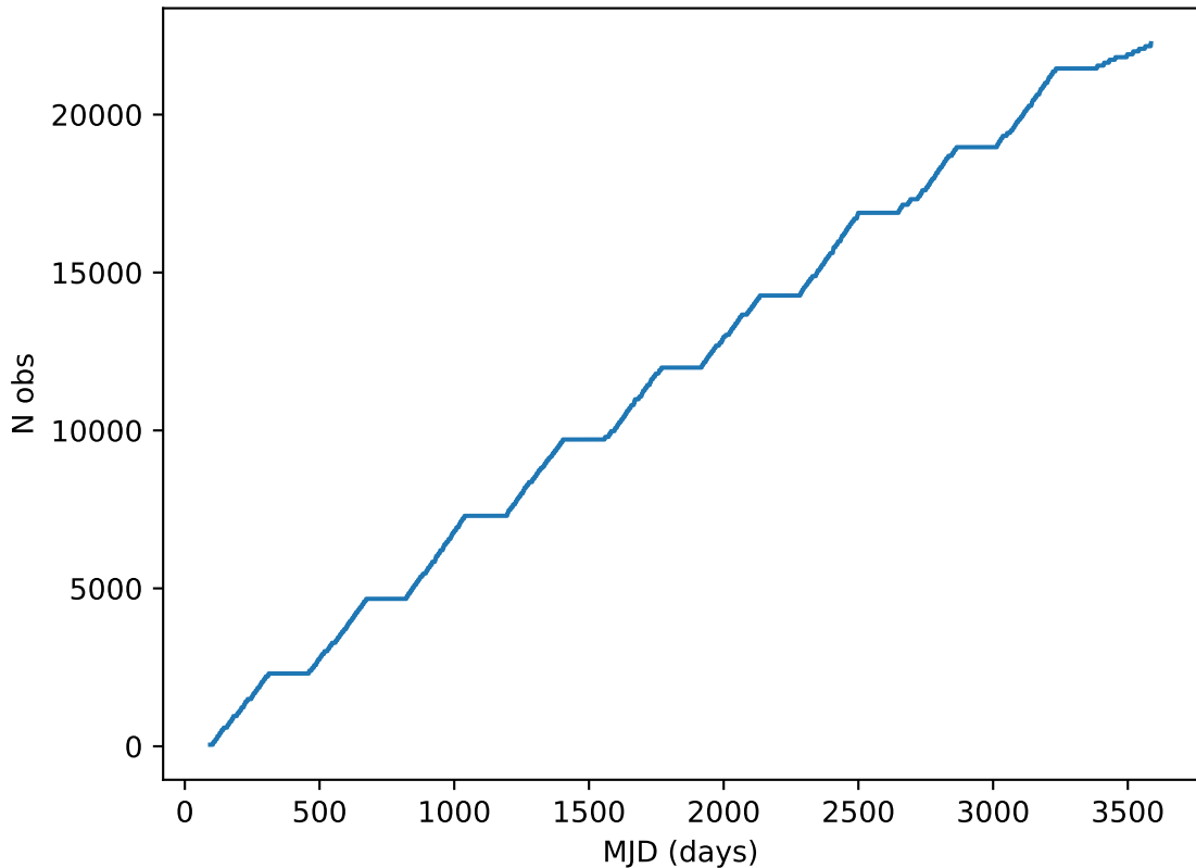
too_elab_r8_d2_griz_v3.4_10yrs all bands: DD:ECDFS Cumulative NVisits
