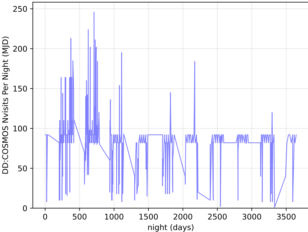
too_elab_r8_d2_griz_v3.4_10yrs all bands: DD: COSMOS Nvisits Per Night
