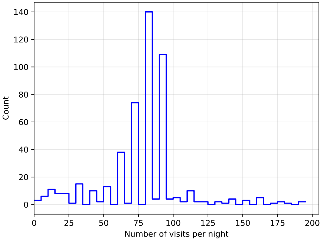
too_elab_r8_d2_griz_v3.4_10yrs all bands: DD: COSMOS NVisitsPerNight
