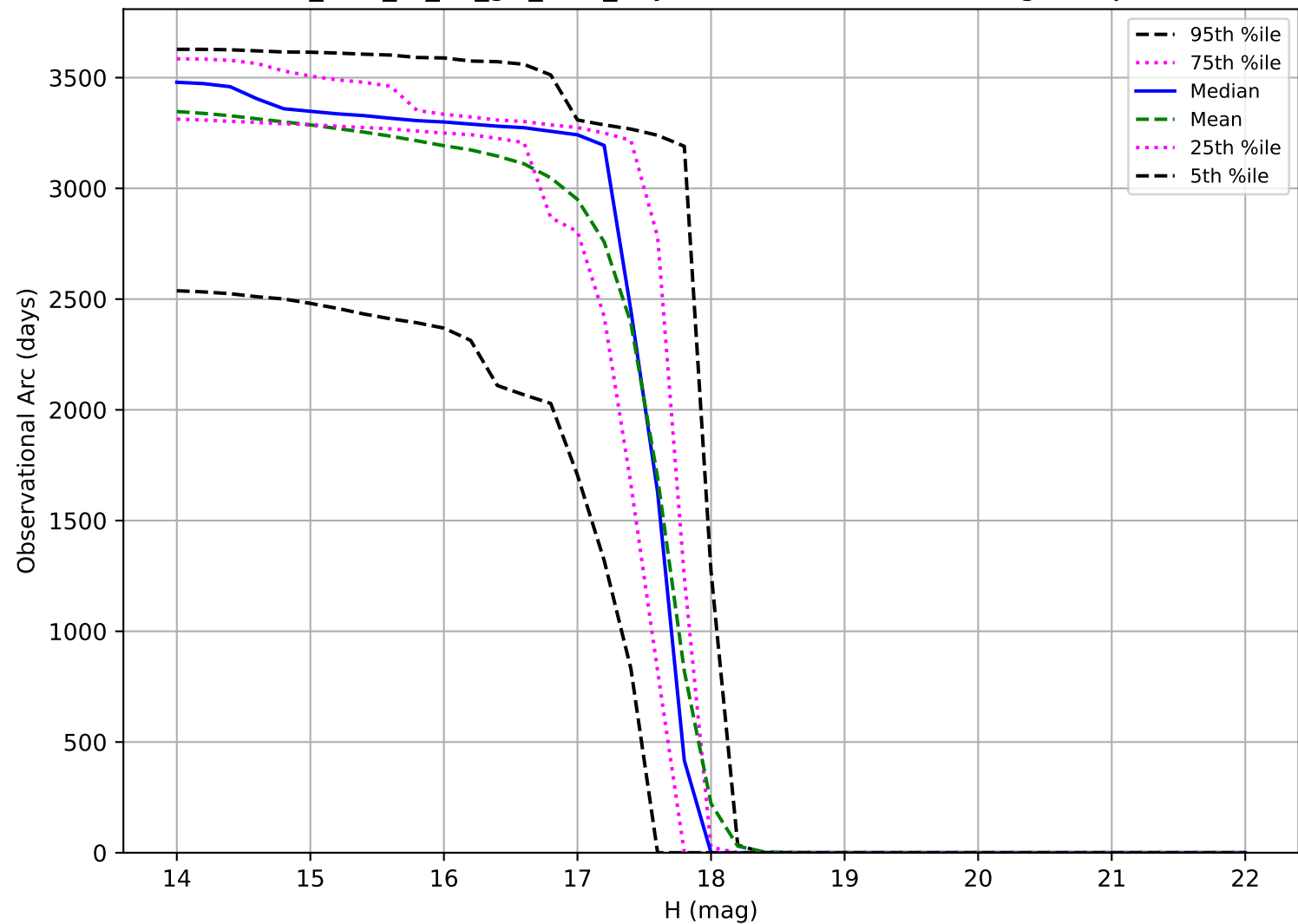
too_elab_r8_d2_giz_v3.4_10yrs: Observational Arc Length Trojan
