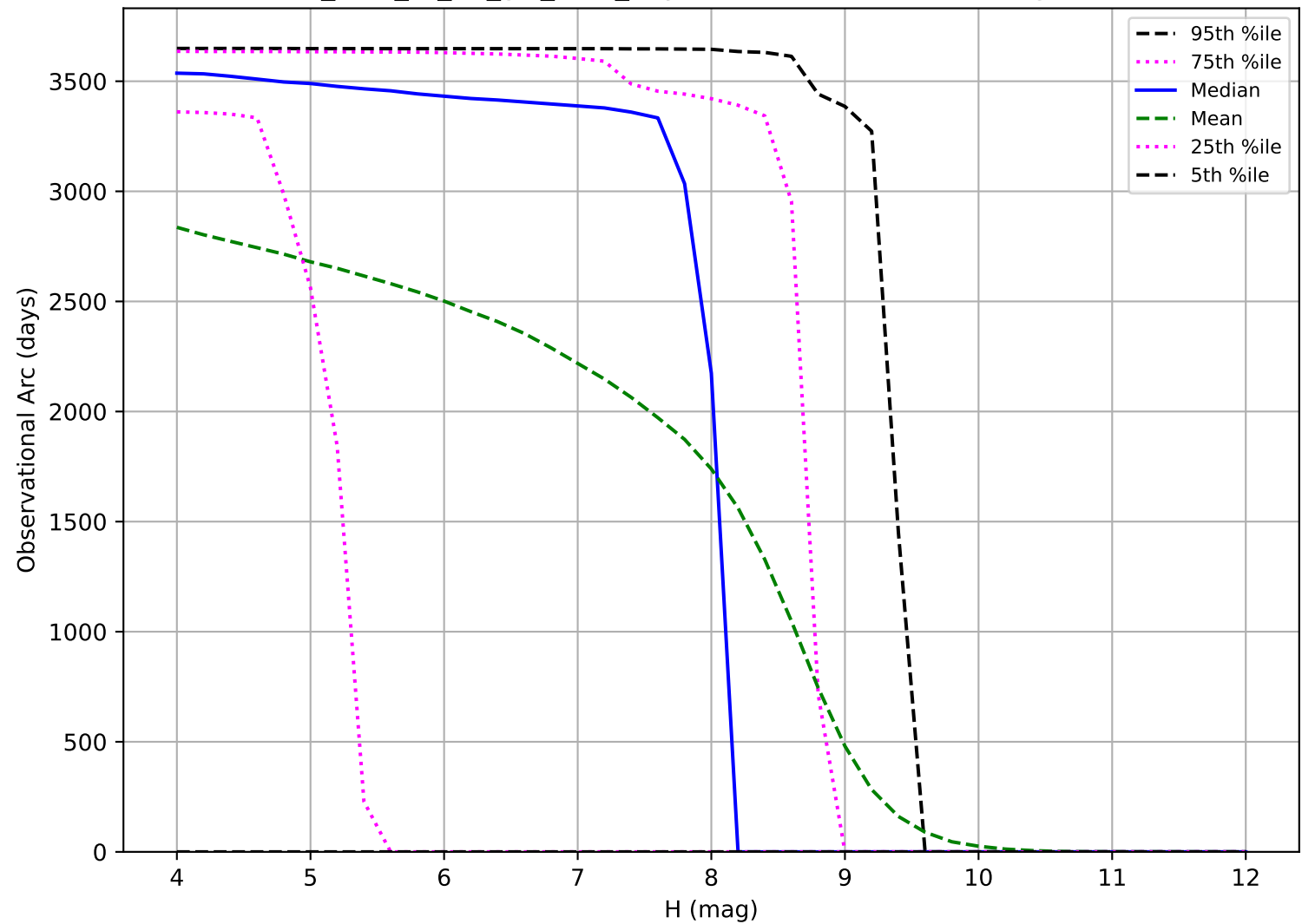
too_elab_r8_d2_giz_v3.4_10yrs: Observational Arc Length TNO
