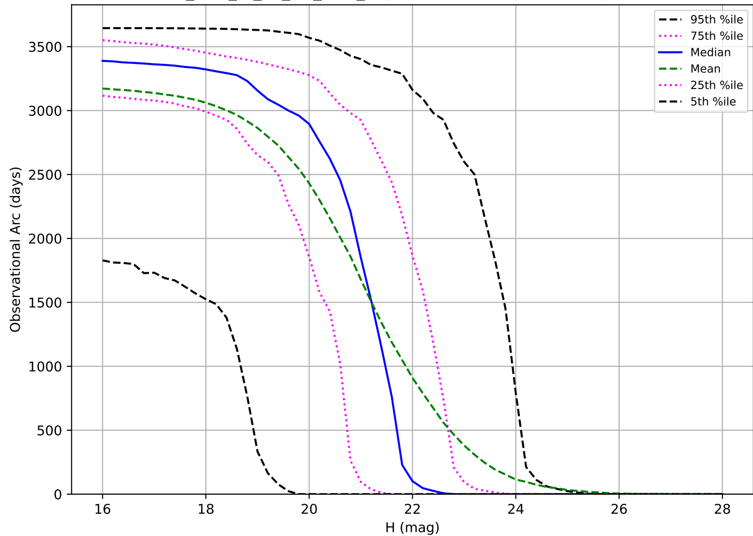
too_elab_r8_d2_giz_v3.4_10yrs: Observational Arc Length NEO
