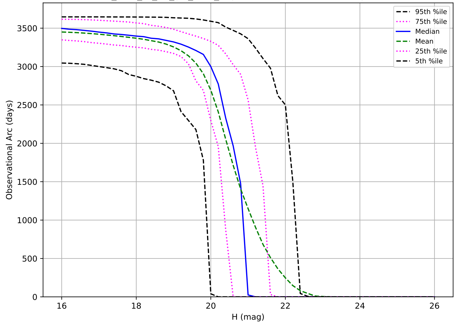
too_elab_r8_d2_giz_v3.4_10yrs: Observational Arc Length MBA
