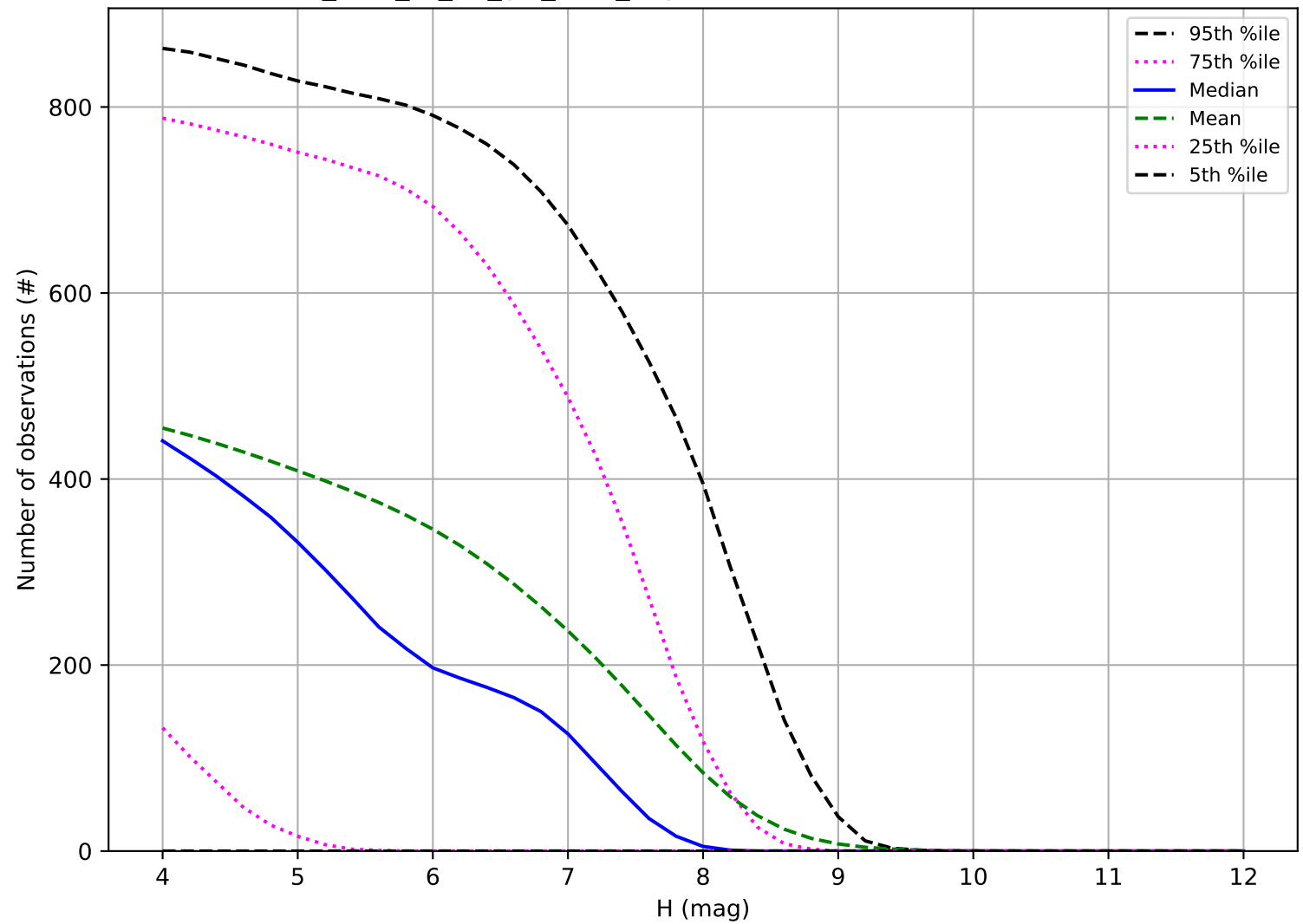
too_elab_r8_d2_giz_v3.4_10yrs: Number of observations TNO
