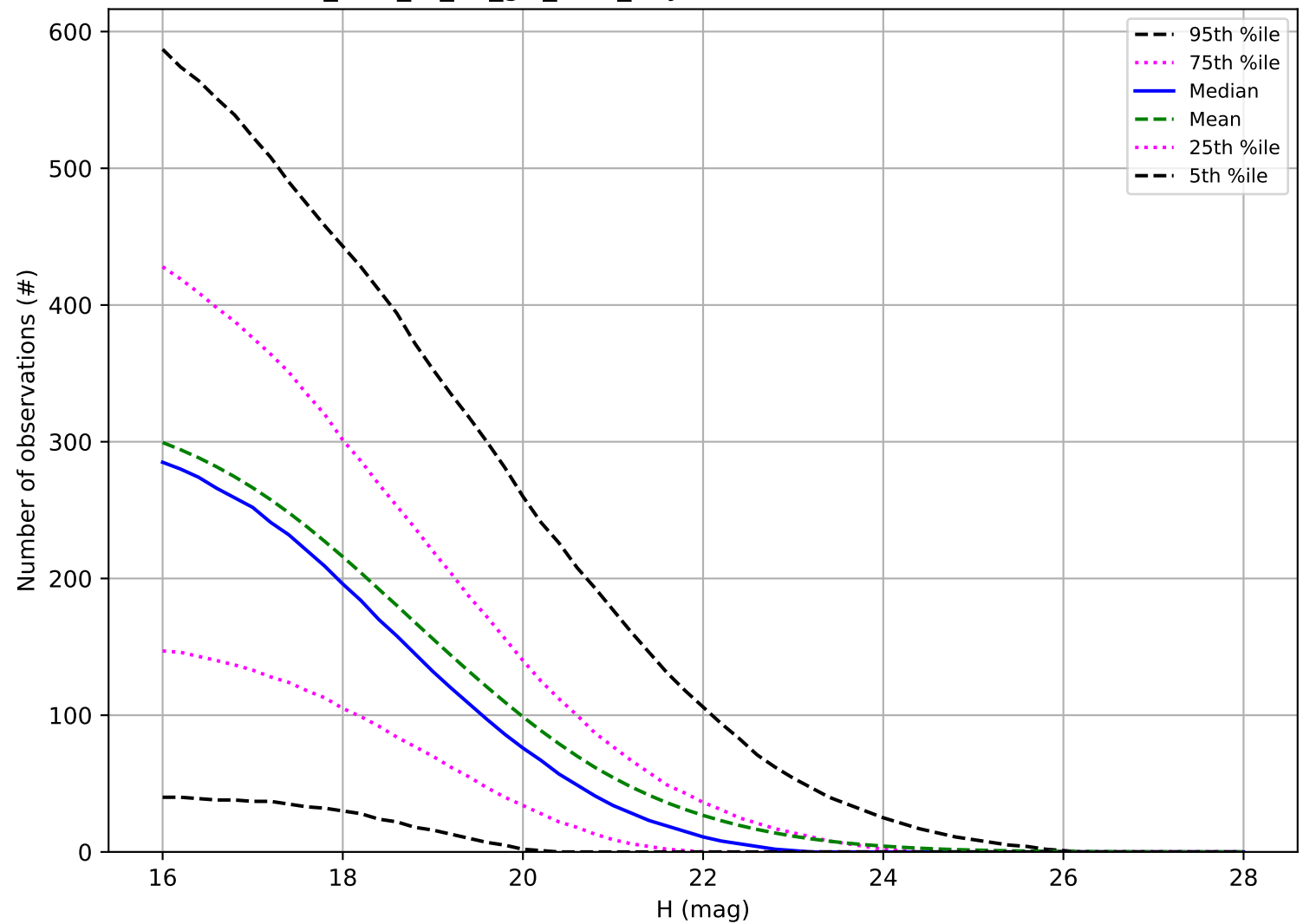
too_elab_r8_d2_giz_v3.4_10yrs: Number of observations PHA
