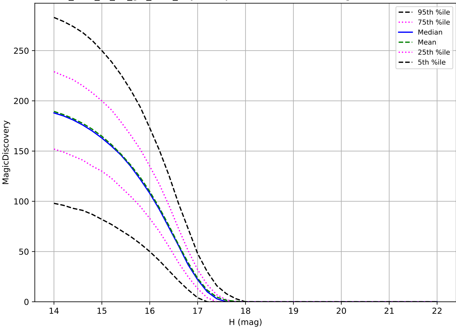
too_elab_r8_d2_giz_v3.4_10yrs: Trojan 6 detections in 60 nights detection loss
