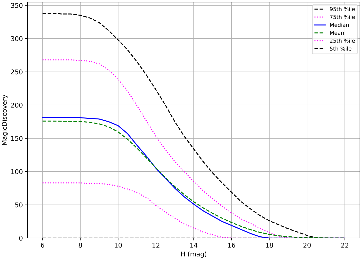
too_elab_r8_d2_giz_v3.4_10yrs: OCC_r5 6 detections in 60 nights detection loss
