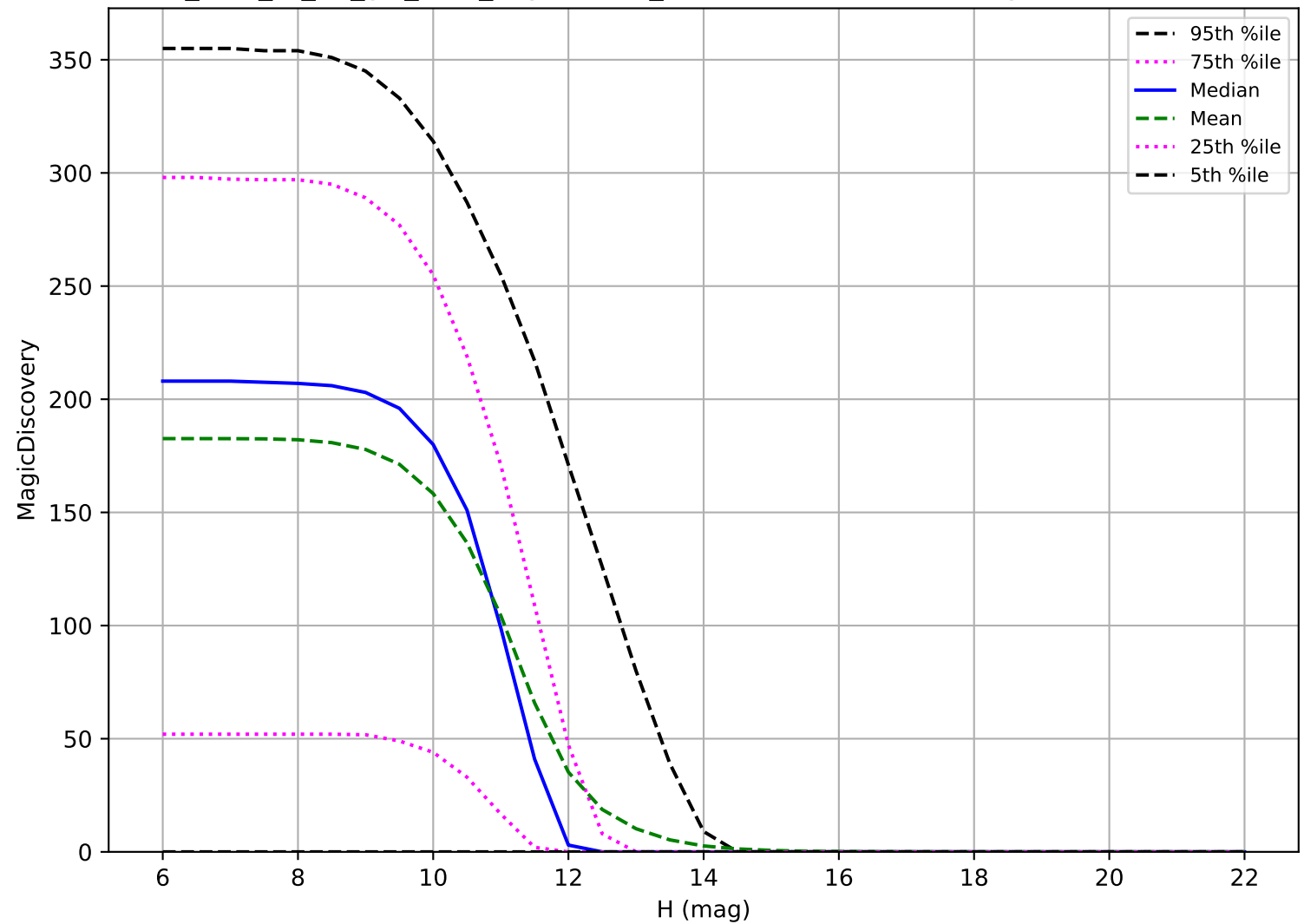
too_elab_r8_d2_giz_v3.4_10yrs: OCC_r20 6 detections in 60 nights detection loss
