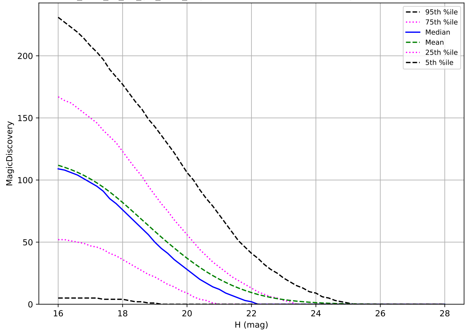
too_elab_r8_d2_giz_v3.4_10yrs: NEO 6 detections in 60 nights detection loss
