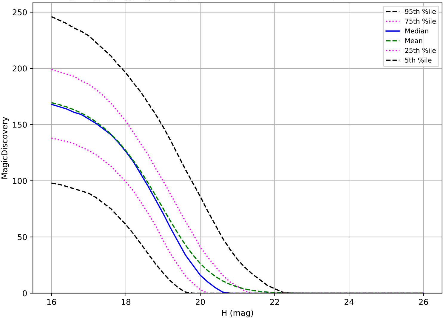
too_elab_r8_d2_giz_v3.4_10yrs: MBA 6 detections in 60 nights detection loss
