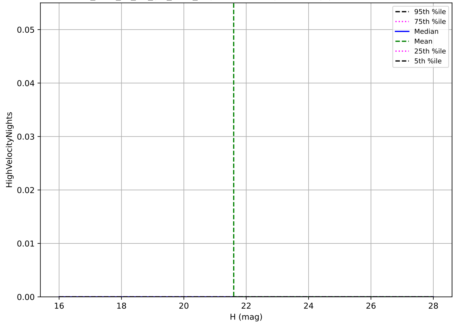
too_elab_r8_d2_giz_v3.4_10yrs: Vatira High velocity pair detection loss
