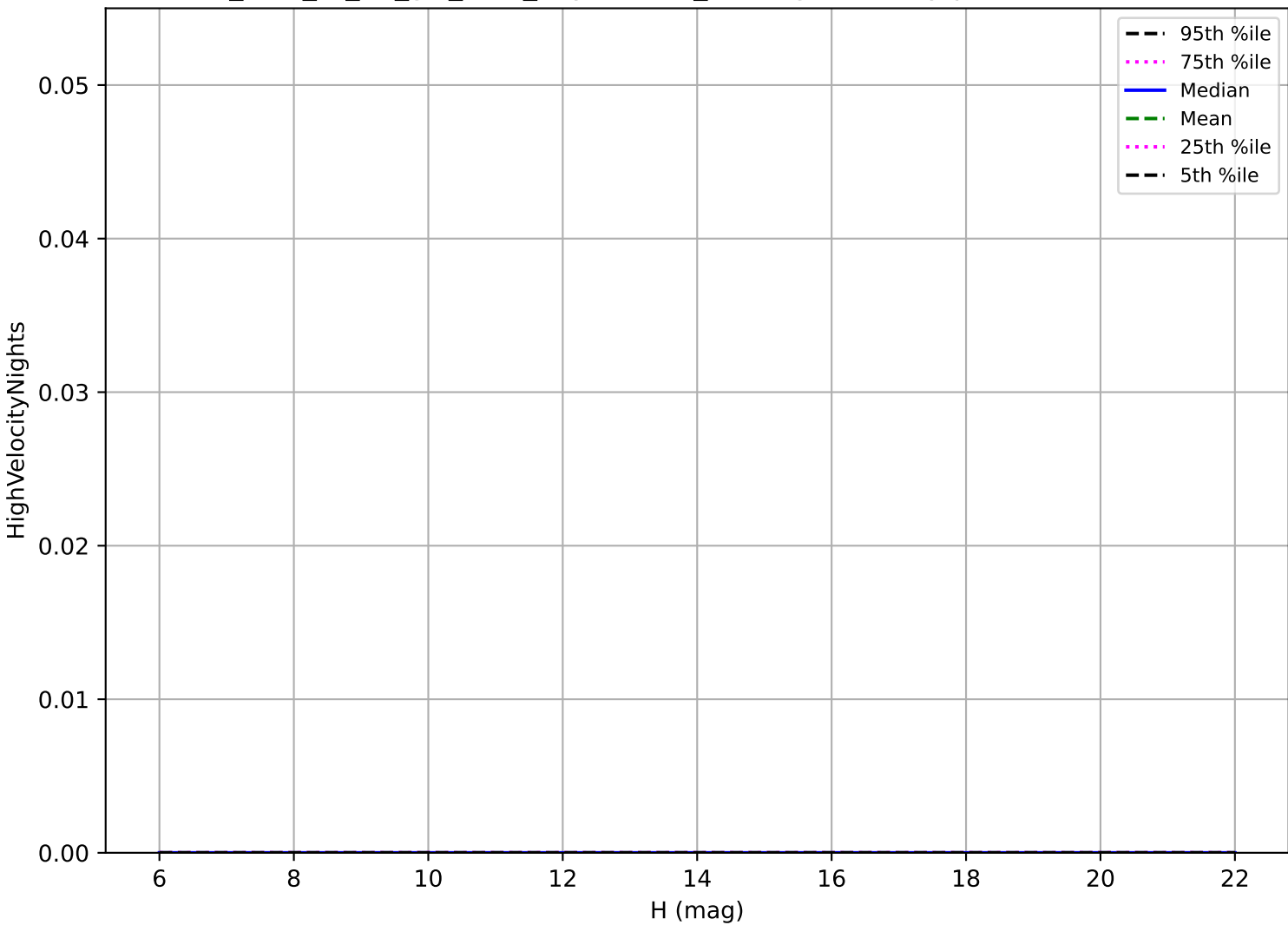
too_elab_r8_d2_giz_v3.4_10yrs: OCC_r20 High velocity pair detection loss
