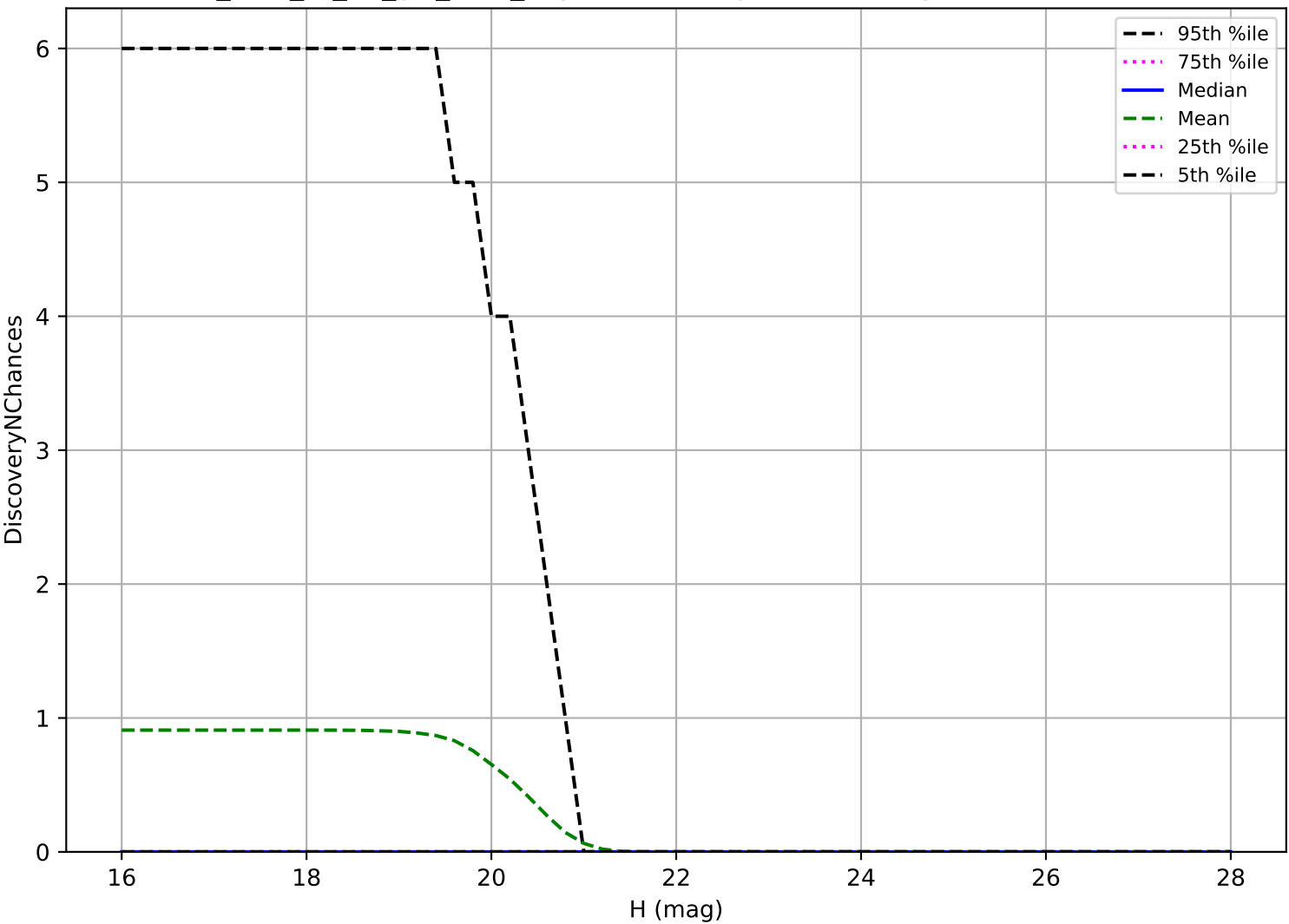
too_elab_r8_d2_giz_v3.4_10yrs: Vatira 3 pairs in 15 nights detection loss
