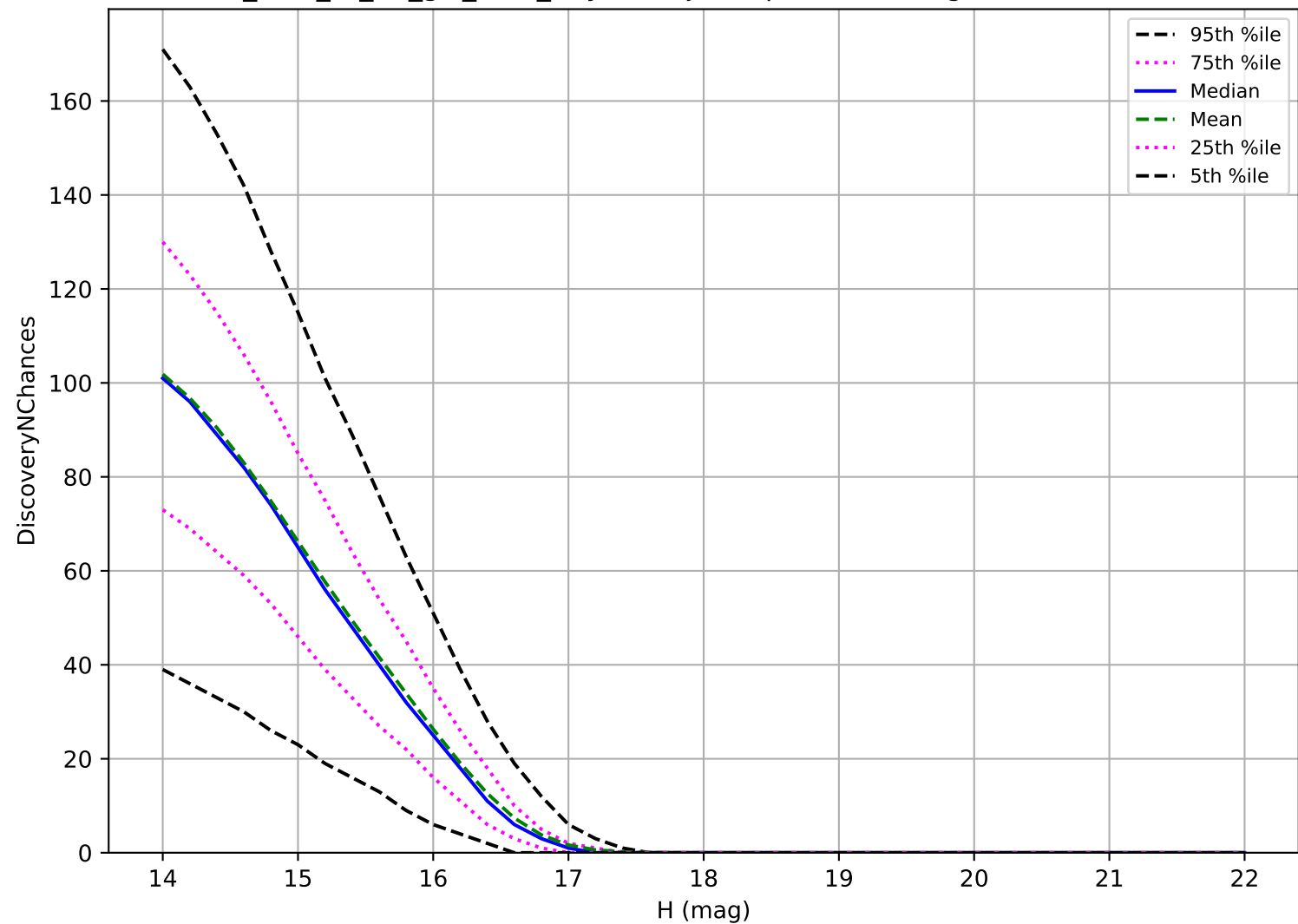
too_elab_r8_d2_giz_v3.4_10yrs: Trojan 3 pairs in 15 nights detection loss
