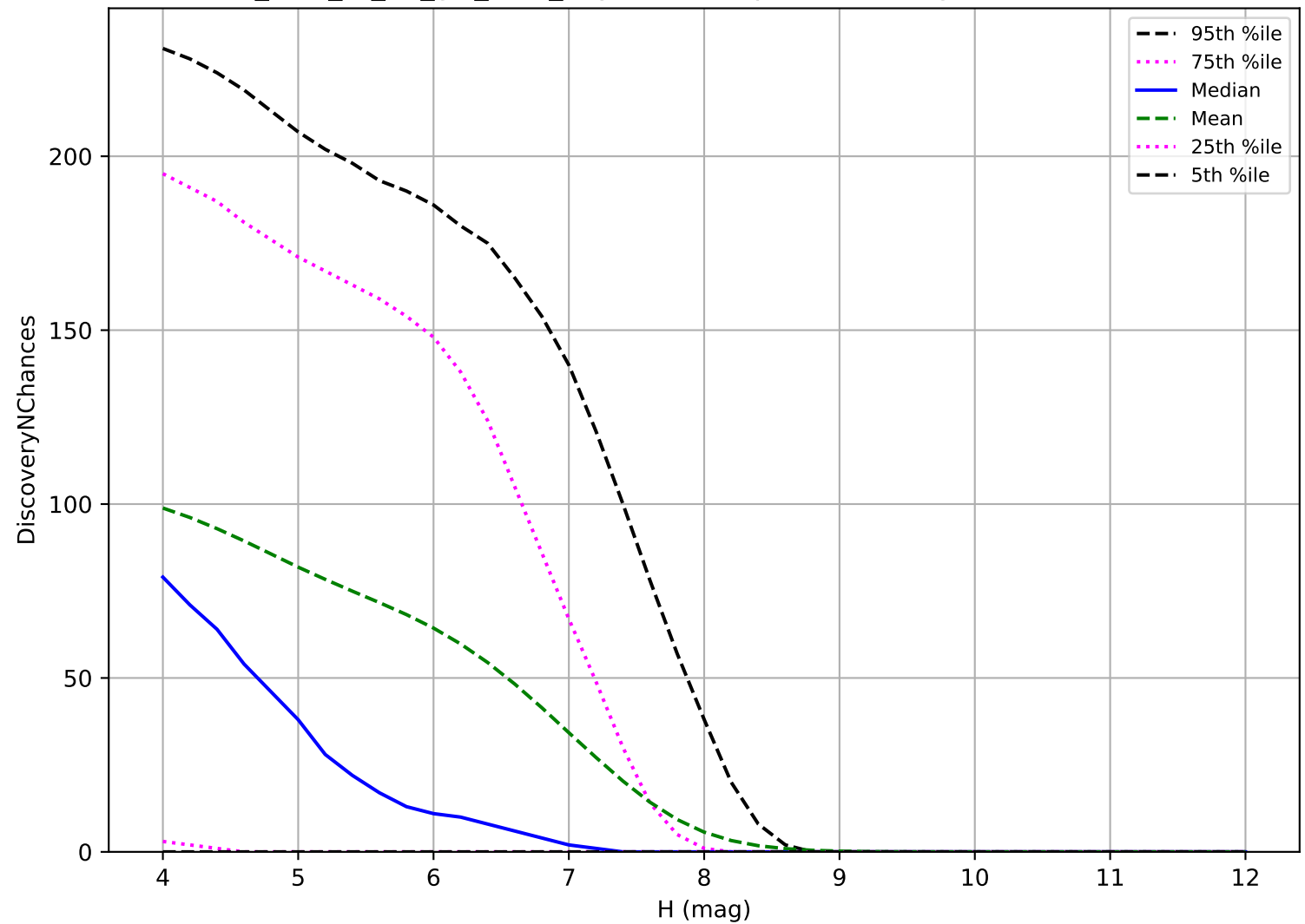
too_elab_r8_d2_giz_v3.4_10yrs: TNO 3 pairs in 15 nights detection loss
