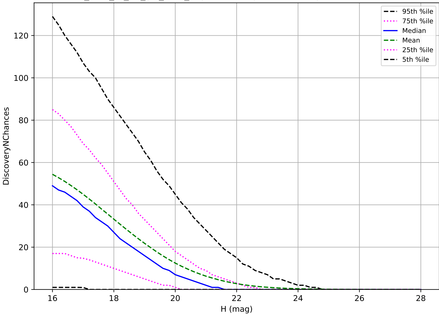
too_elab_r8_d2_giz_v3.4_10yrs: PHA 3 pairs in 15 nights detection loss
