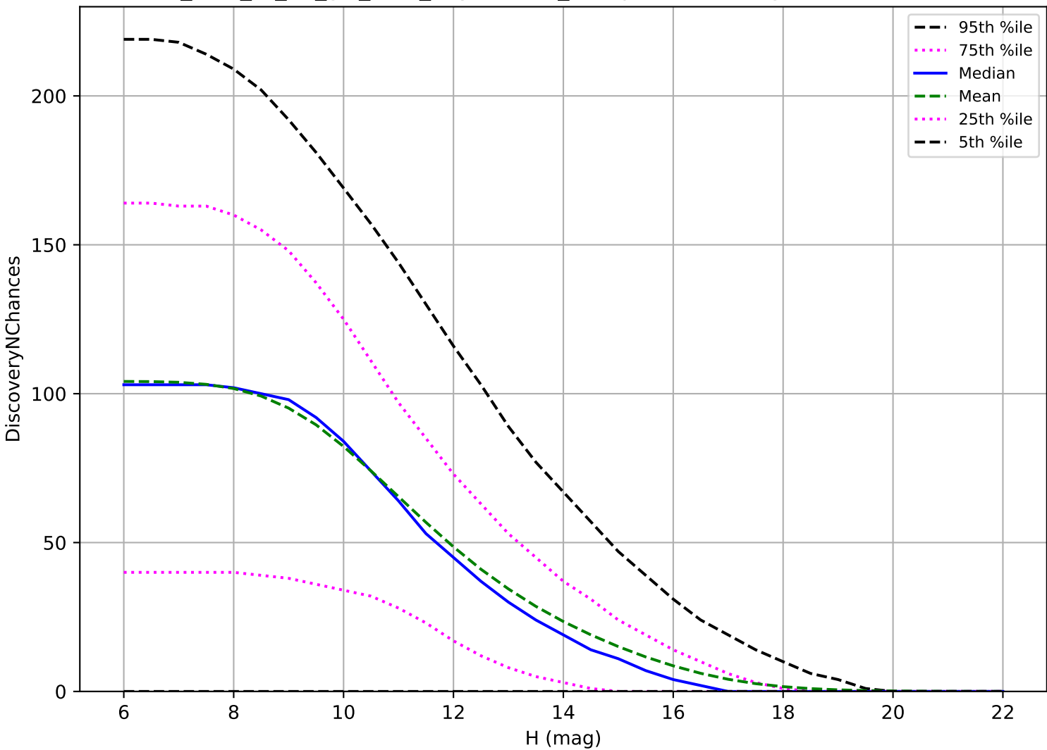
too_elab_r8_d2_giz_v3.4_10yrs: OCC_r5 3 pairs in 15 nights detection loss
