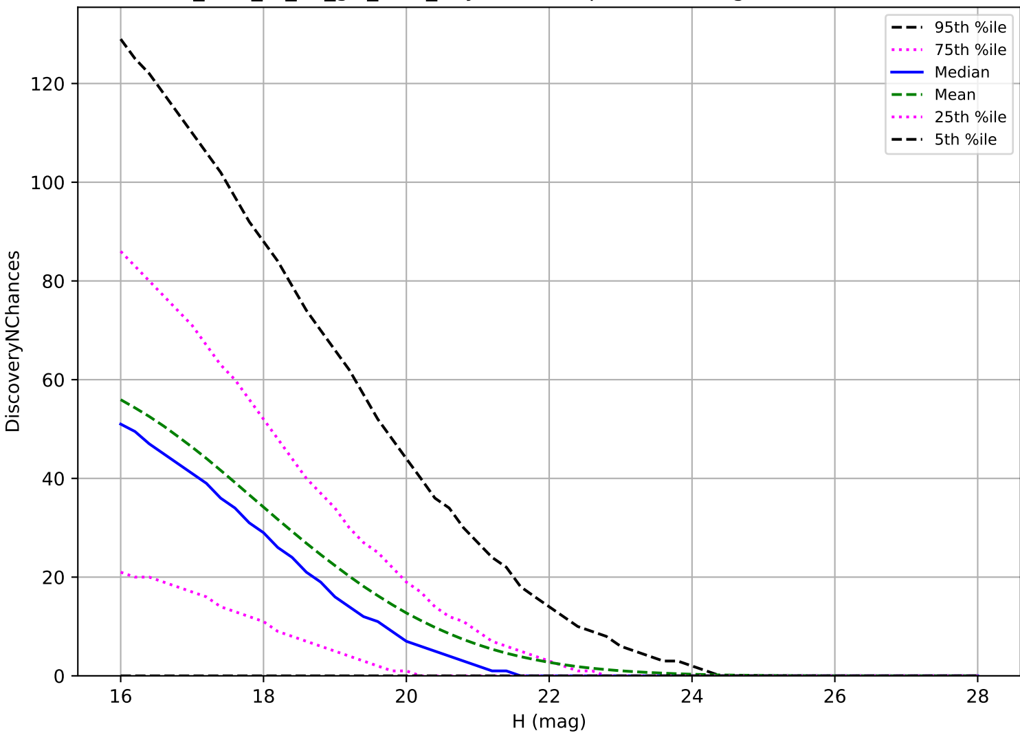
too_elab_r8_d2_giz_v3.4_10yrs: NEO 3 pairs in 15 nights detection loss
