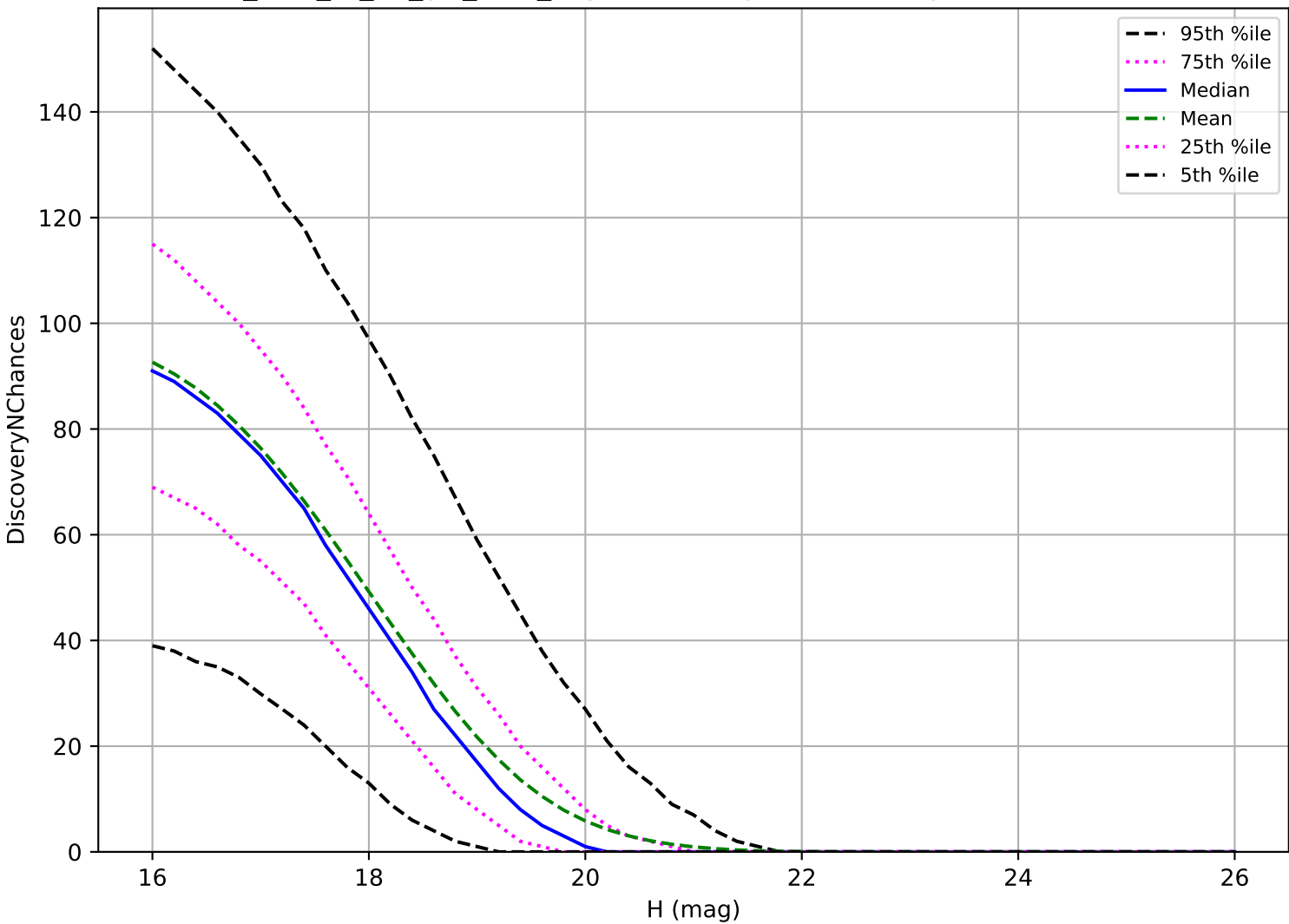
too_elab_r8_d2_giz_v3.4_10yrs: MBA 3 pairs in 15 nights detection loss
