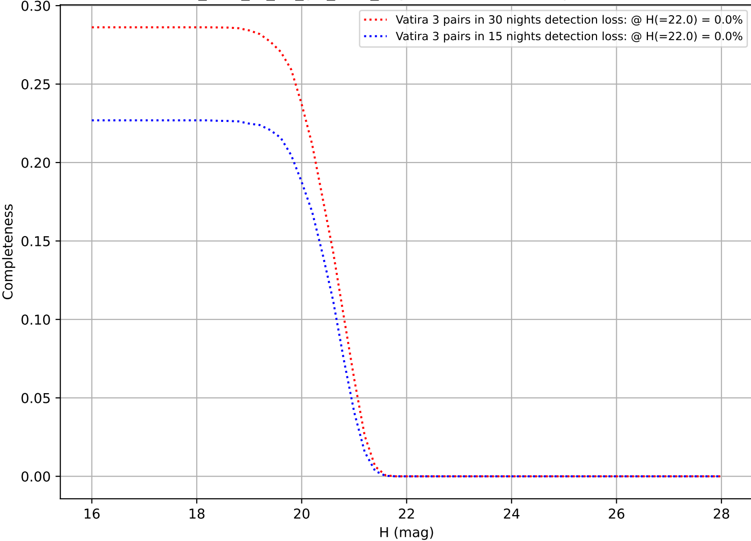
too_elab_r8_d2_giz_v3.4_10yrs: DifferentialCompleteness
