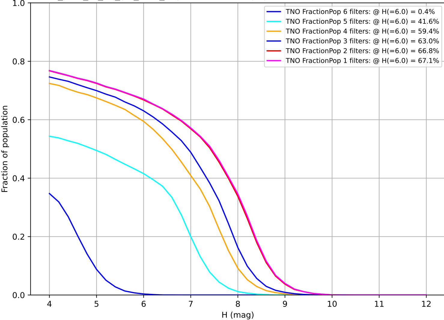
too_elab_r8_d2_giz_v3.4_10yrs: Fraction of population with colors in X filters TNO
