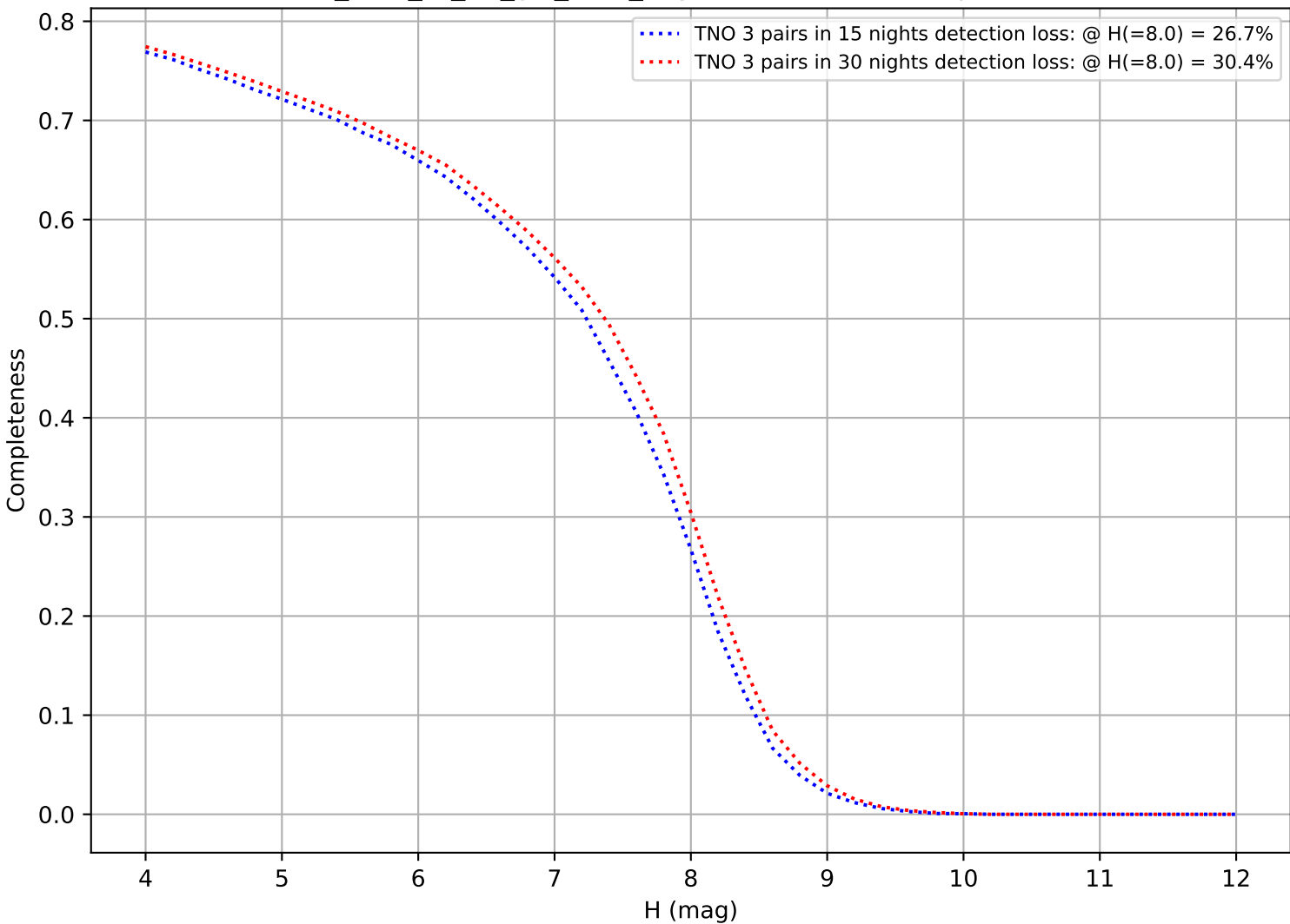
too_elab_r8_d2_giz_v3.4_10yrs: DifferentialCompleteness
