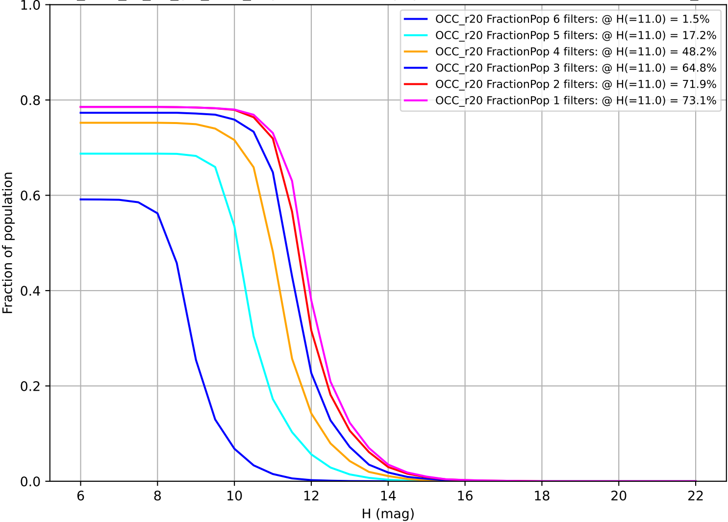
too_elab_r8_d2_giz_v3.4_10yrs: Fraction of population with colors in X filters OCC_r20
