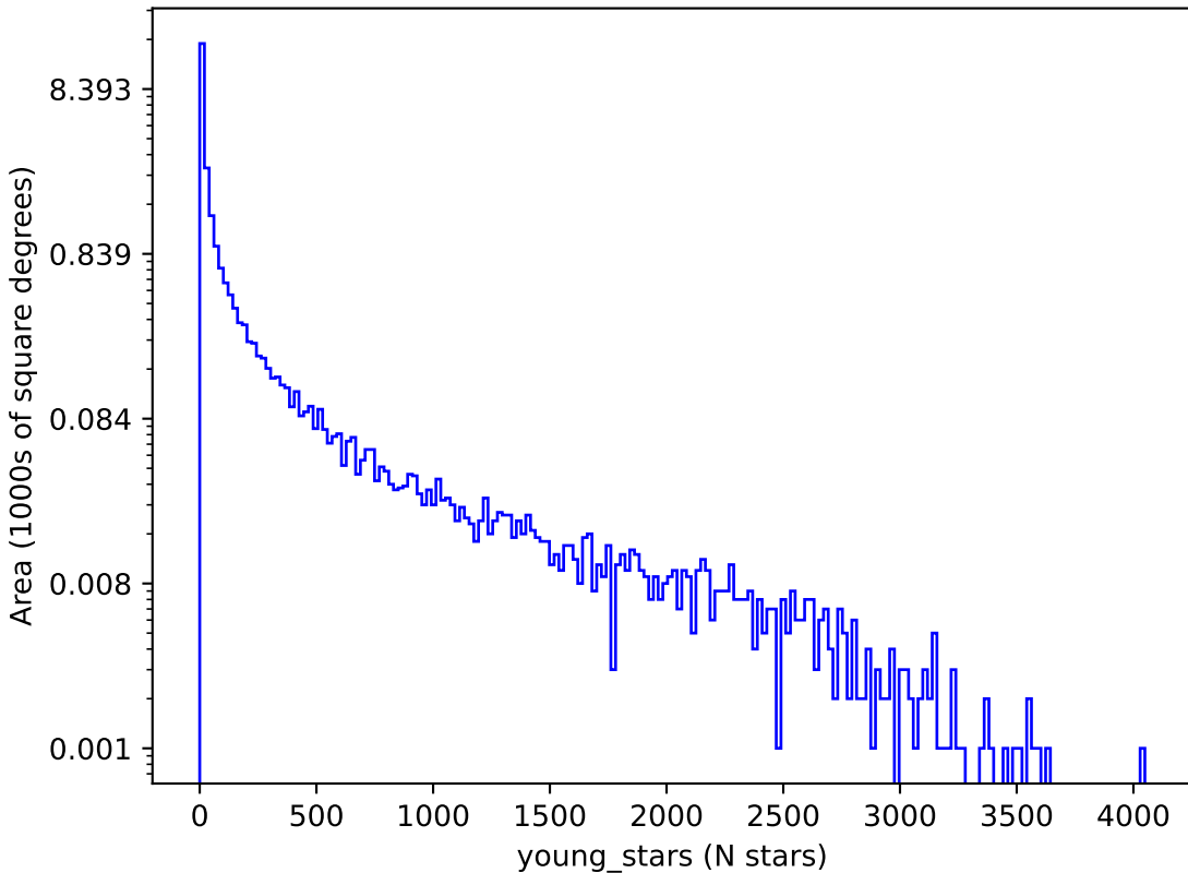
too_elab_r8_d2_giz_v3.4_10yrs : young_stars
