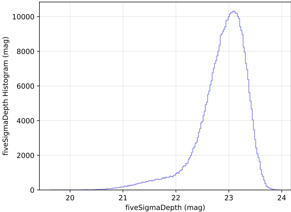
too_elab_r8_d2_giz_v3.4_10yrs z: fiveSigmaDepth Histogram
