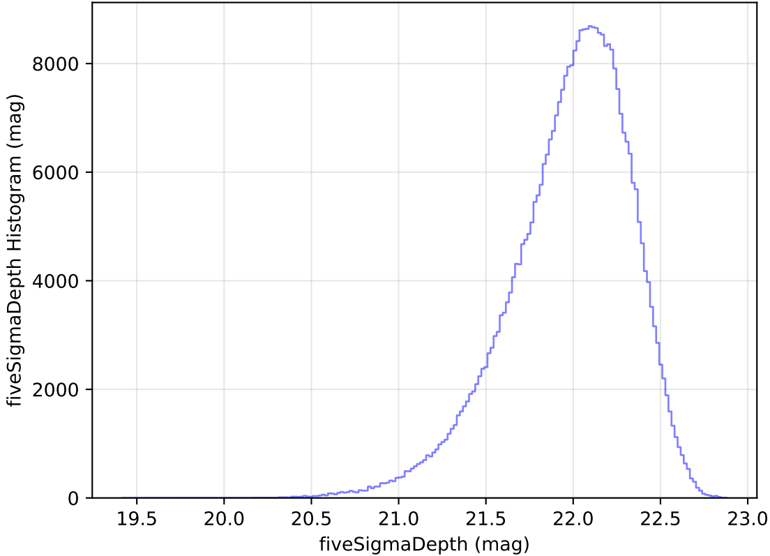
too_elab_r8_d2_giz_v3.4_10yrs y: fiveSigmaDepth Histogram
