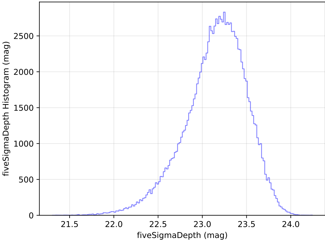
too_elab_r8_d2_giz_v3.4_10yrs u: fiveSigmaDepth Histogram
