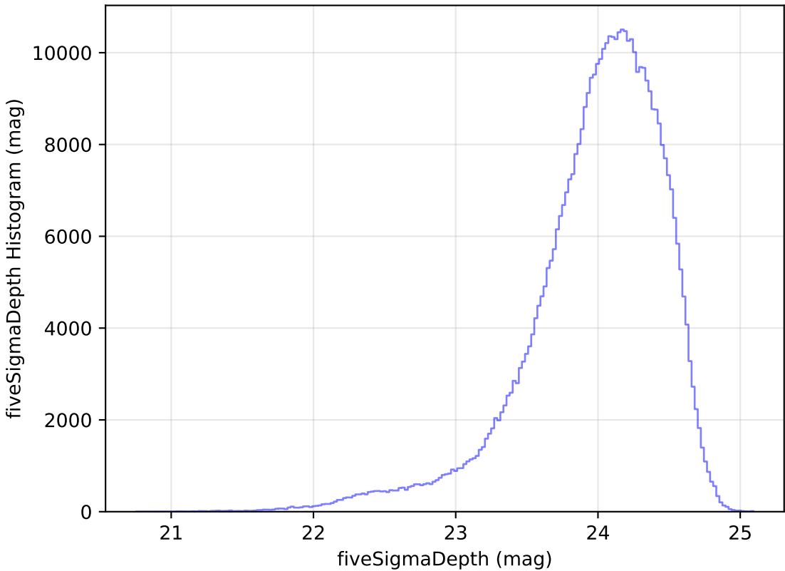
too_elab_r8_d2_giz_v3.4_10yrs r: fiveSigmaDepth Histogram
