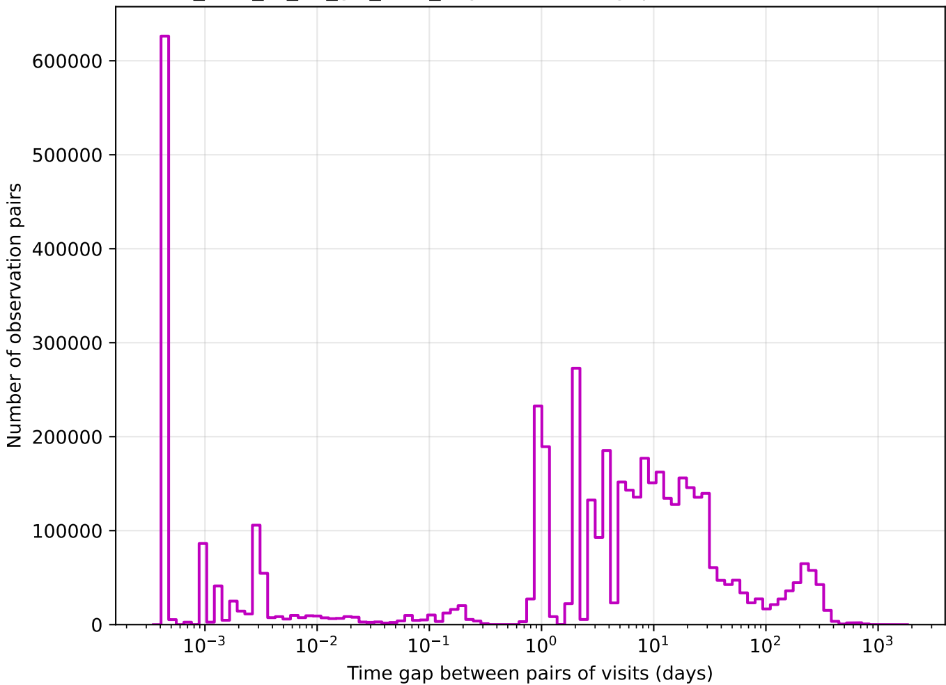
too_elab_r8_d2_giz_v3.4_10yrs z band: Tgaps observationStartMJD
