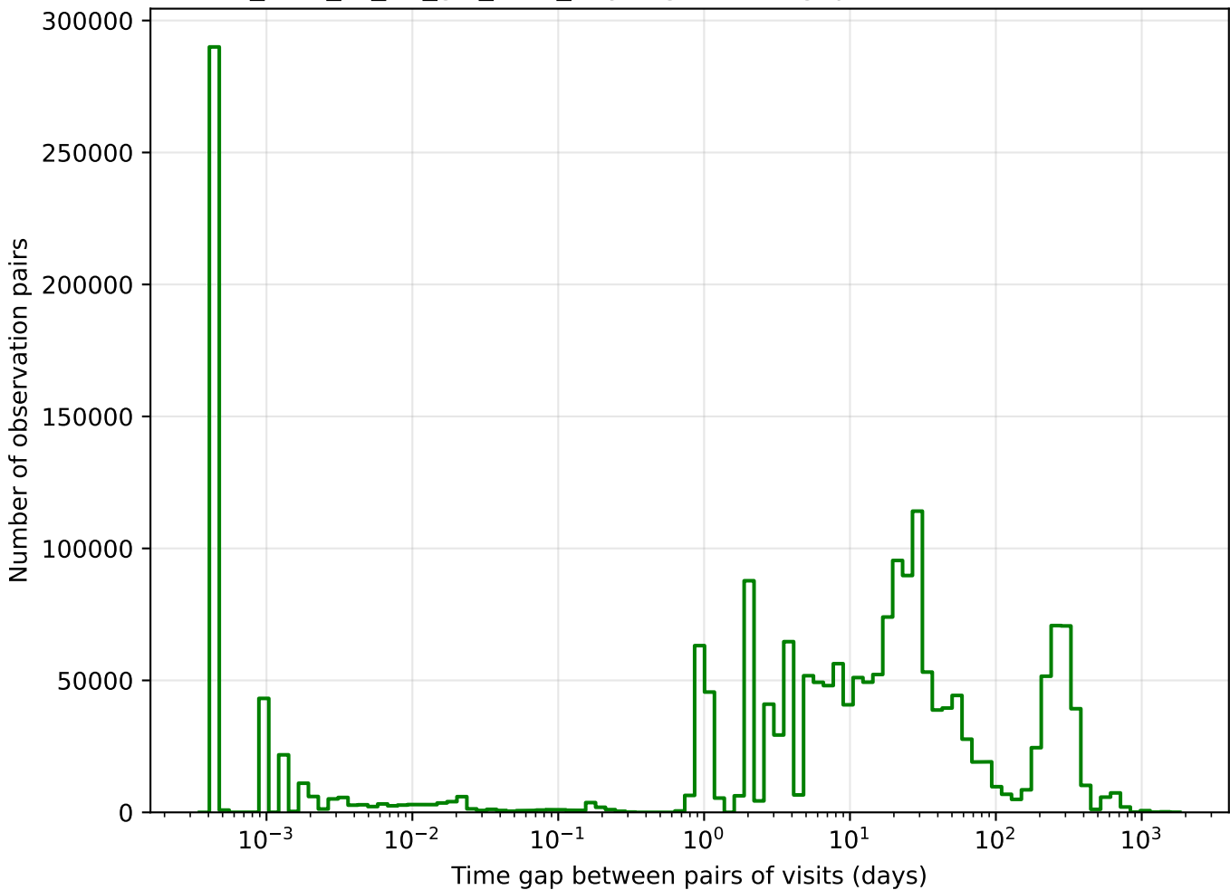
too_elab_r8_d2_giz_v3.4_10yrs g band: Tgaps observationStartMJD
